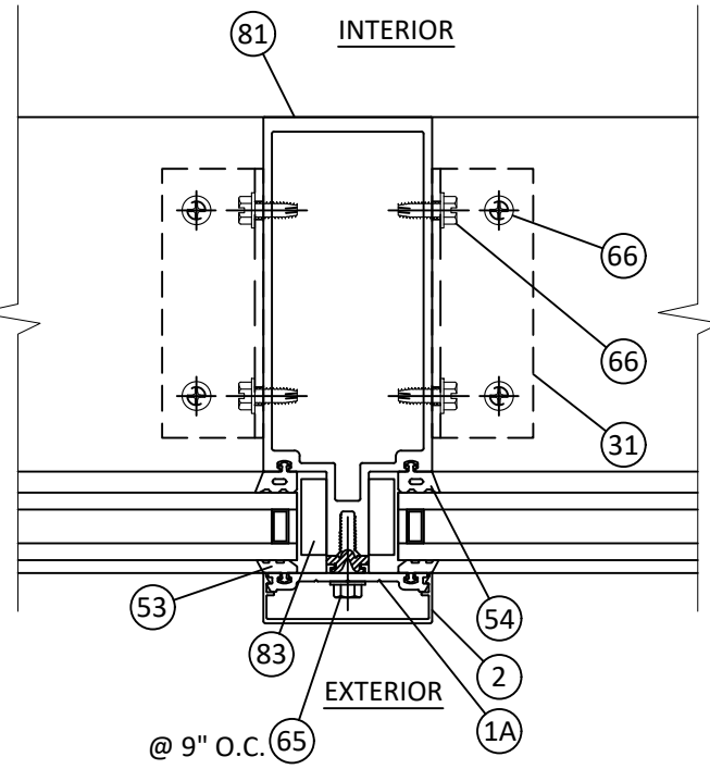
3 4.1 HORIZONTAL SECTION VERTICAL MULLION PRESSURE PLATE W/ SHEAR CLIP
