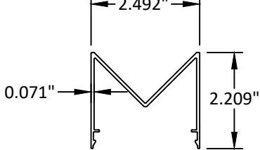
CORNER INT. COVER 6063-T5
