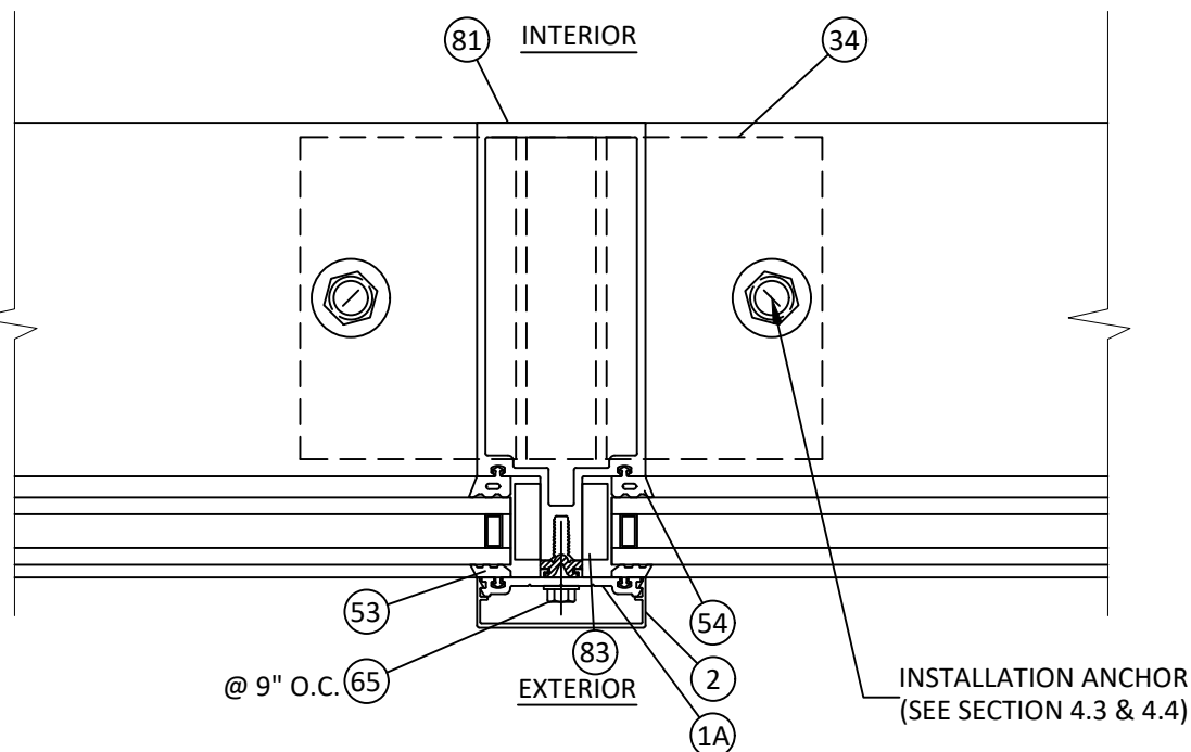
6 4.1 HORIZONTAL SECTION T-ANCHOR AT VERTICAL MULLION TYPICAL
