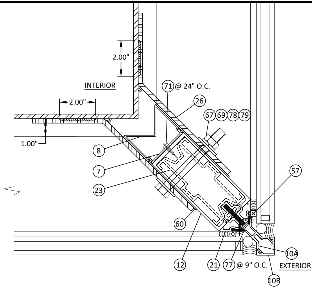
3 HORIZONTAL SECTION 4.2 VERTICAL CORNER MULLION SSG W/ WIND LOAD ANCHOR
