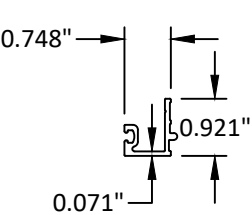
1/4" GLAZING ADAPTOR 6063-T5
