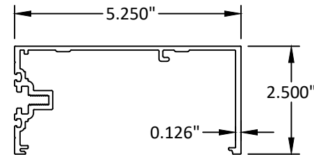
14 OPEN BACK HEAD/SILL/HORIZONTAL 6063-T6
