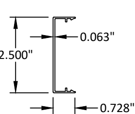
FACE COVER 6063-T5
