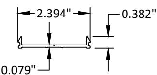
CORNER INT. BASE 6063-T5
