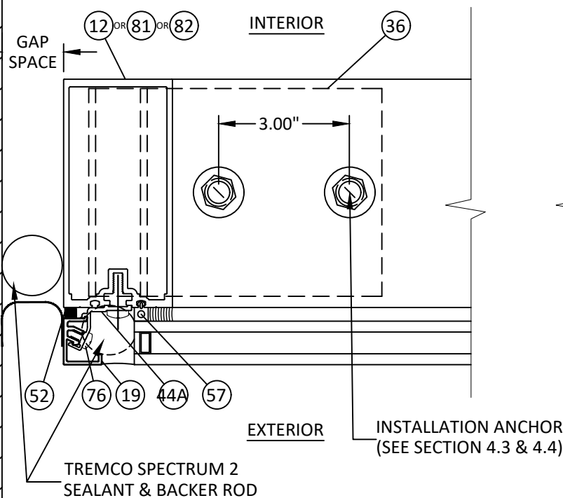
5 4.1 HORIZONTAL SECTION F-ANCHOR AT JAMB MULLION TYPICAL
