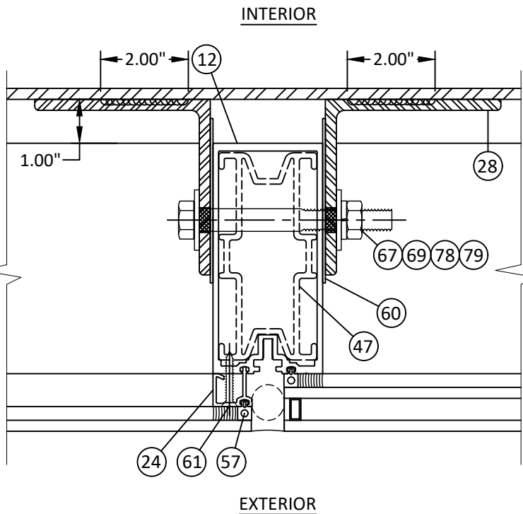
2 HORIZONTAL SECTION 4.2 VERTICAL MULLION SSG W/ WIND LOAD ANCHOR
