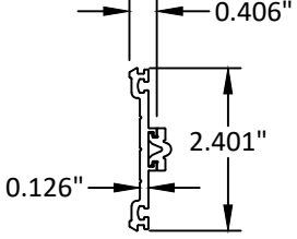
PRESSURE PLATE 6063-T5
