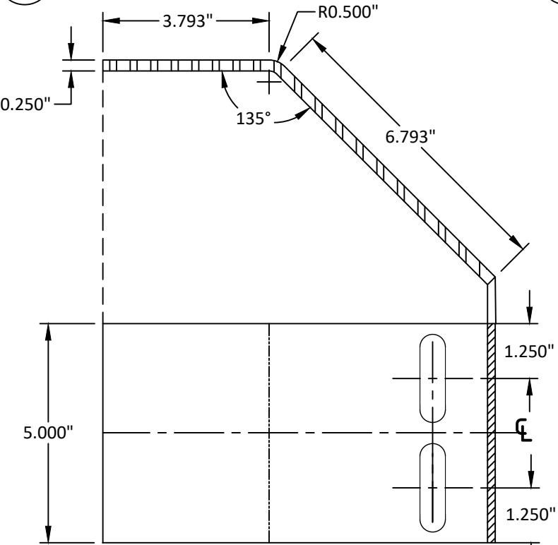
26 CORNER WINDLOAD ANCHOR A36 STEEL (PRIMED)
