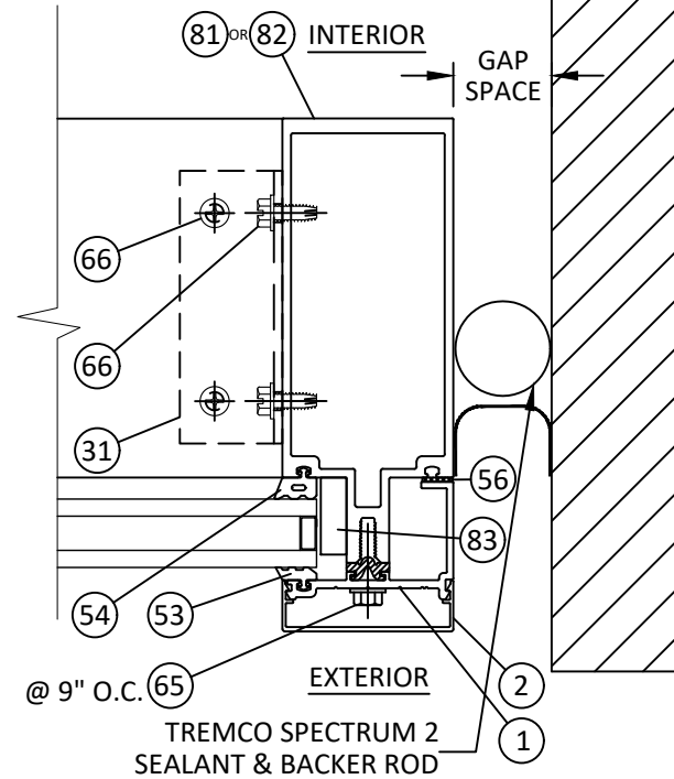
4 4.1 HORIZONTAL SECTION JAMB MULLION PRESSURE PLATE W/ SHEAR CLIP
