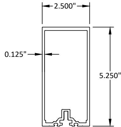
21 CORNER GLAZING ADAPTOR 6063-T5
