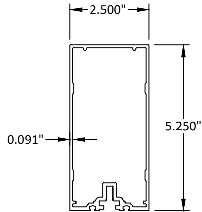
13 VERTICAL/HORIZONTAL MULLION 6063-T6
