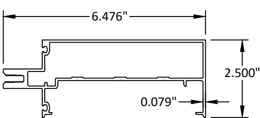
HORIZONTAL MULLION 6063-T5
