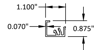
19 PERIMTER TRIM (FIELD) 6063-T5
