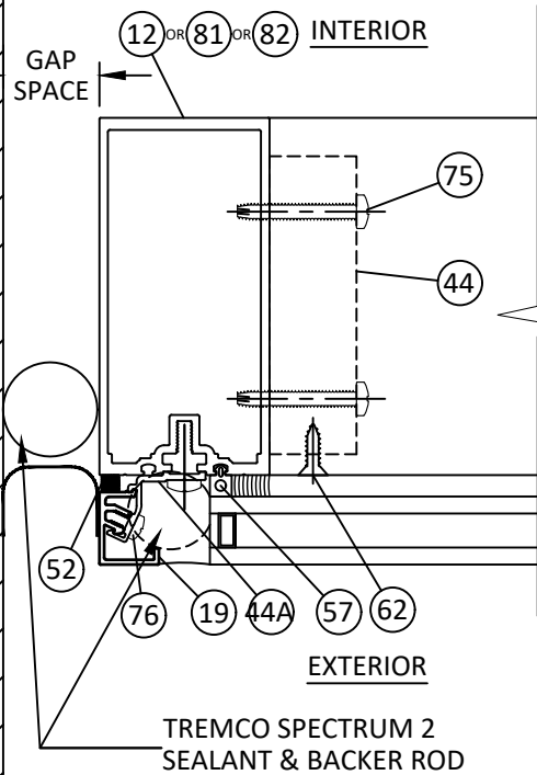
1 4.1 HORIZONTAL SECTION JAMB MULLION SSG W/ SHEAR BLOCK
