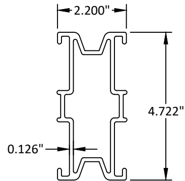
23 47 SPLICE SLEEVE PROFILE 6063-T5
