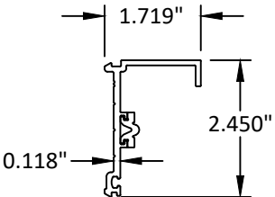
PERIMETER PRESSURE PLATE 6063-T5
